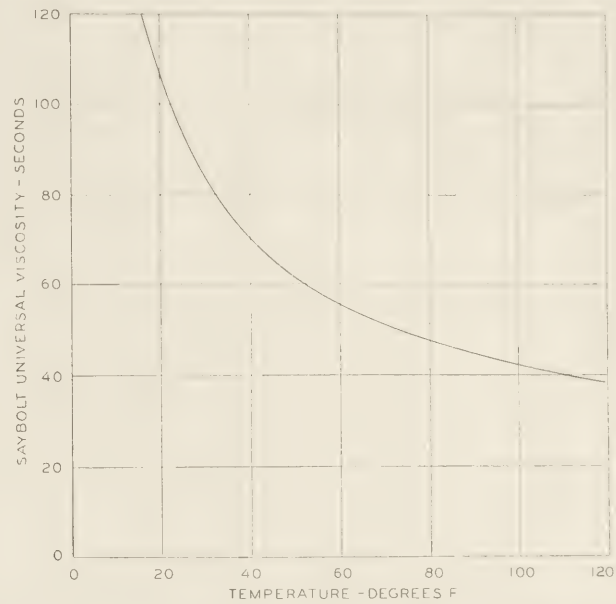
FIGURE 14.—VISCOSITY CURVE FOR THE 50-50 BLEND OF KEROSENE AND REFRIGERATION OIL USED IN THE DAMPING UNITS.
